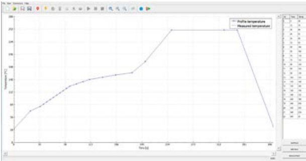
Predefined process temperature profile
